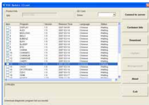
Fig.2-7 Download interface
